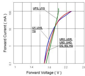
Forward Voltage vs. Forward Current
